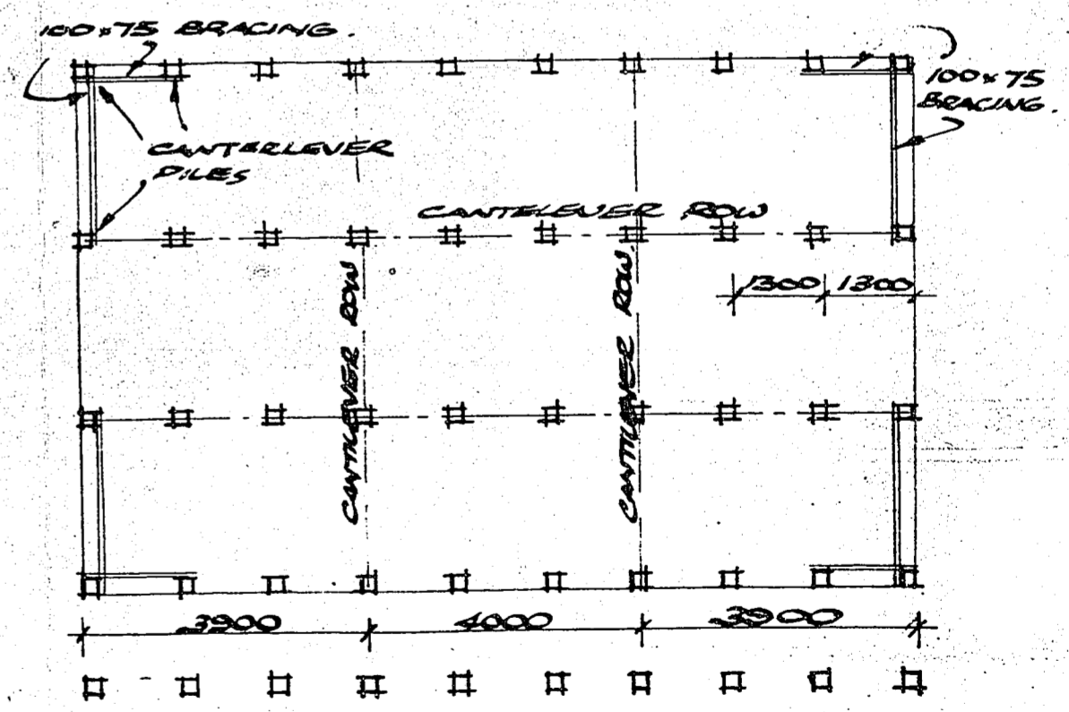
PILE LAYOUT
