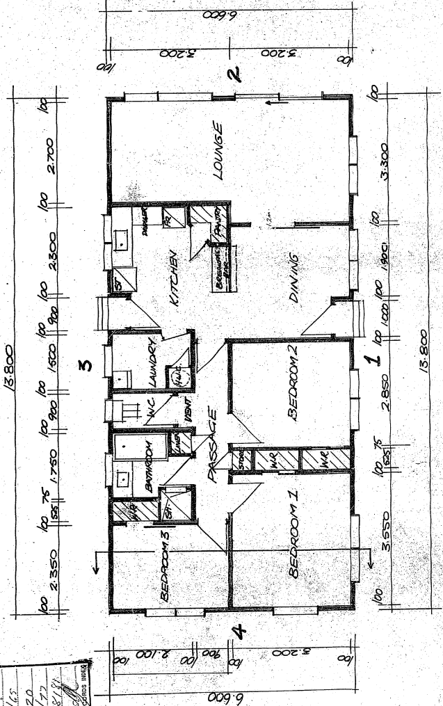
FLOOR PLAN
